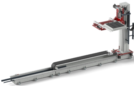
ASRS FOR BATTERY MODULES
